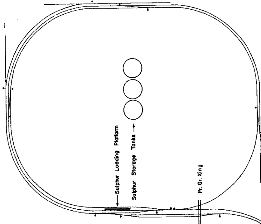
DUVAL SULPHUR PLANT Scale 1" = 200'
